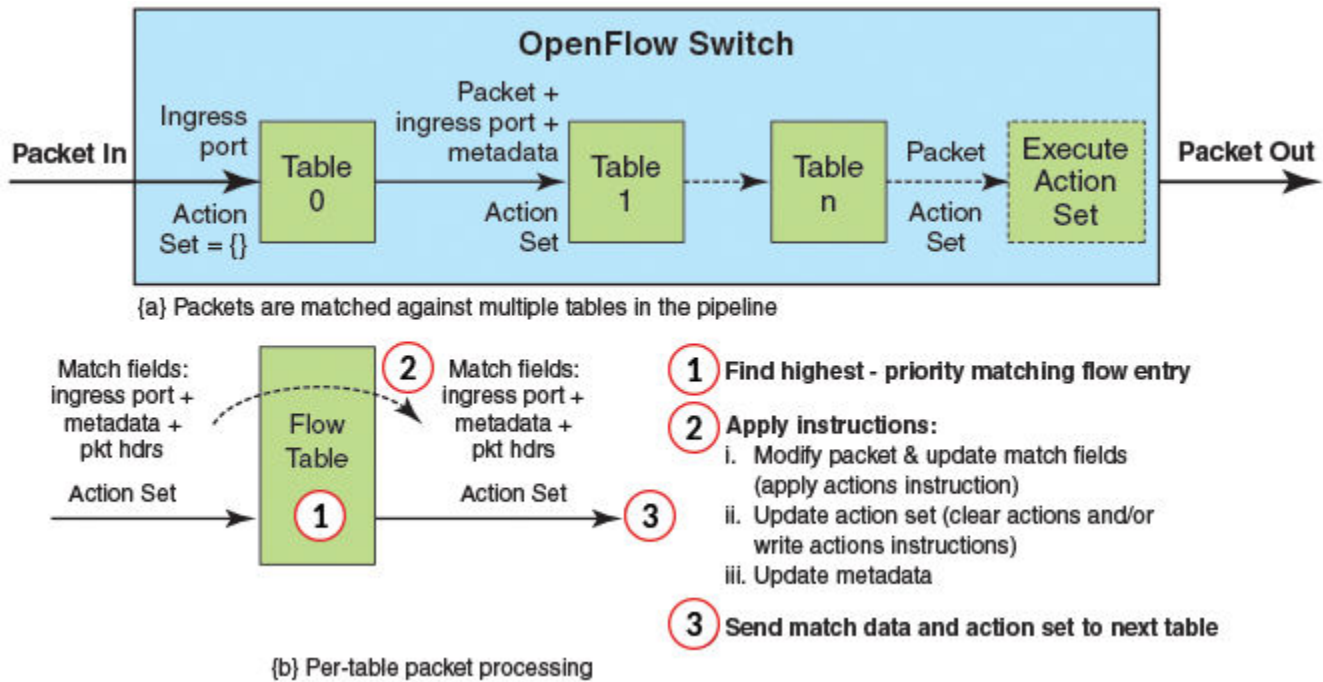
FIGURE 6 Pipeline Processing
